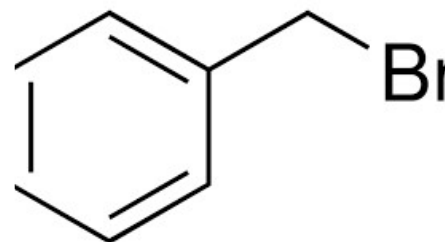
Benzyl bromide
